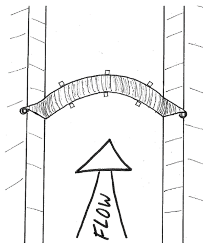
Figure 4: Fiber Roll Plan View
