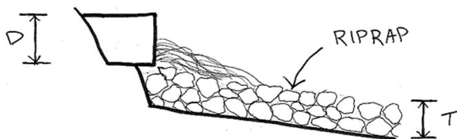
Figure 30: Rock Apron – Section View
