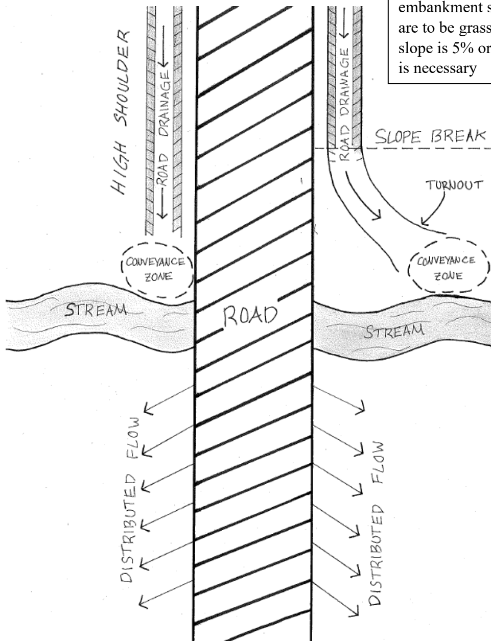
Figure 27: Conveyance Zones
