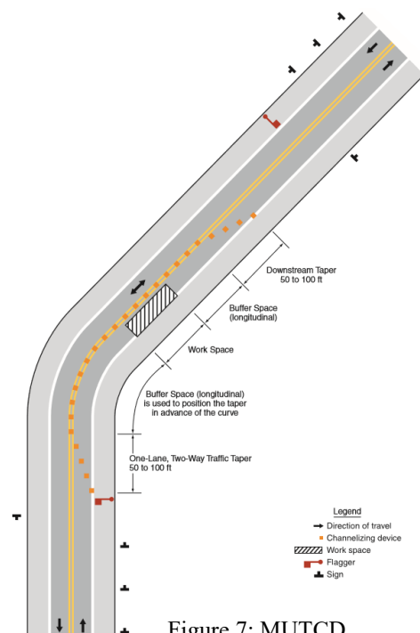
Figure 7: MUTCD Fig.6H-10
