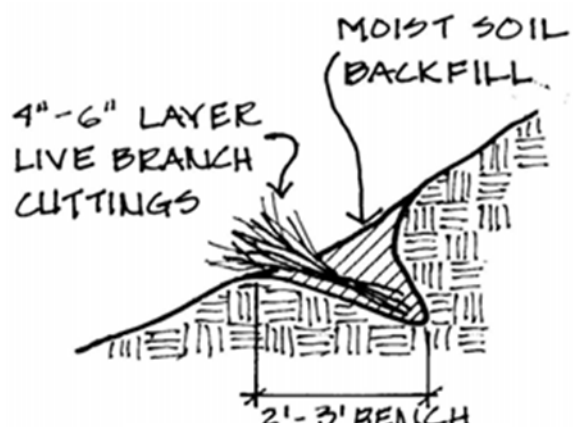
Figure 41: Brush Layering
