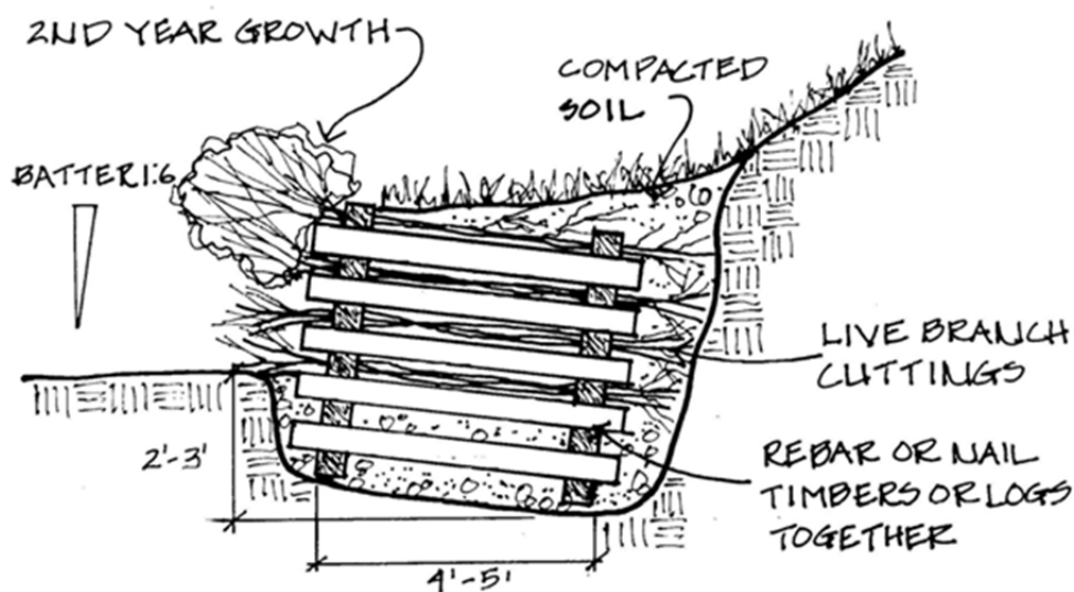
Figure 37: Live Crib
