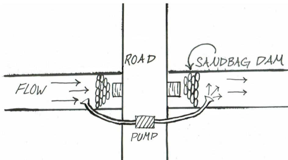
Figure 22: Culvert Installation
