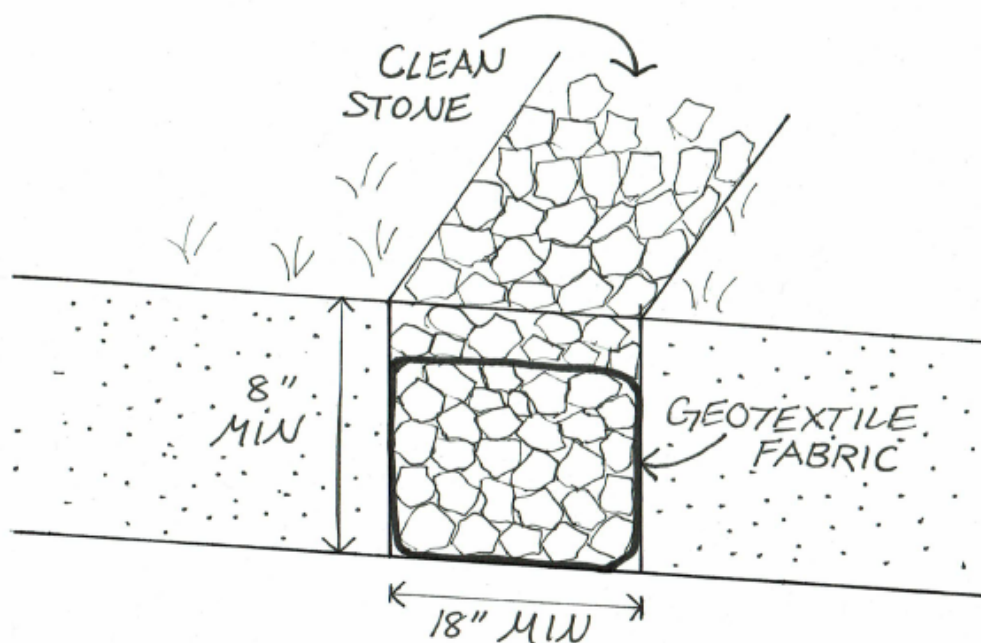
Figure 18: Infiltration Trench
