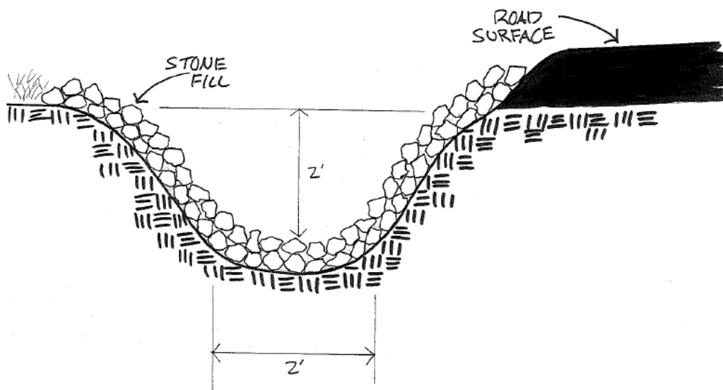
Figure 13: Stone lined ditch
