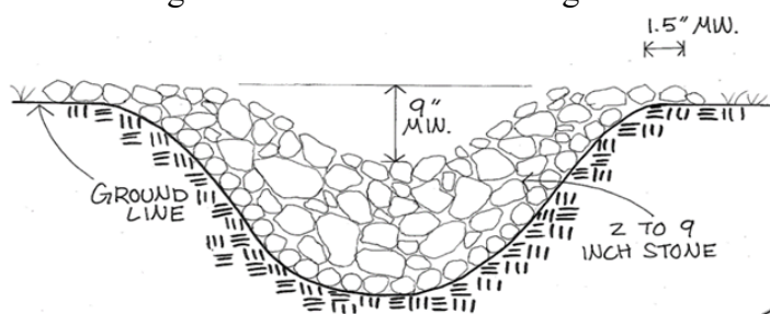
Figure 14: Section view perpendicular to channel
