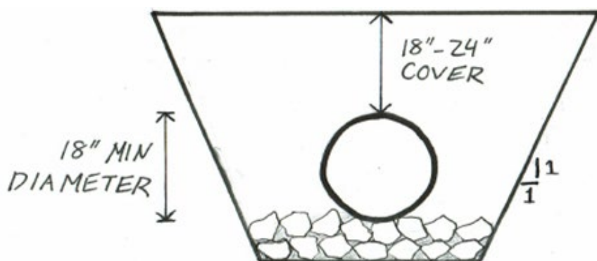
Figure 26: Culvert Installation
