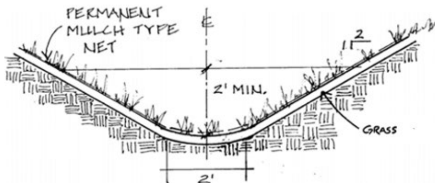
Figure 12: Grass lined ditch
